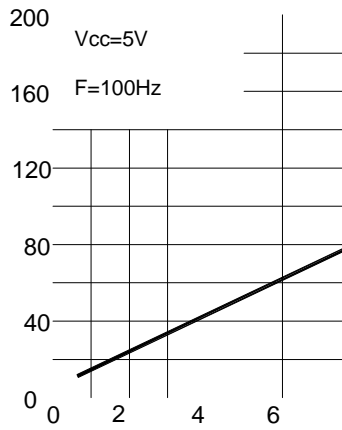
FIG.3 Rise And Fall Time Vs. Load Resistance
