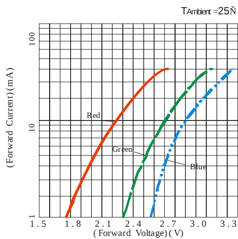
Volt-Ampere Characteristics
