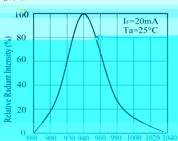
Fig.2 Spectral Distribution
